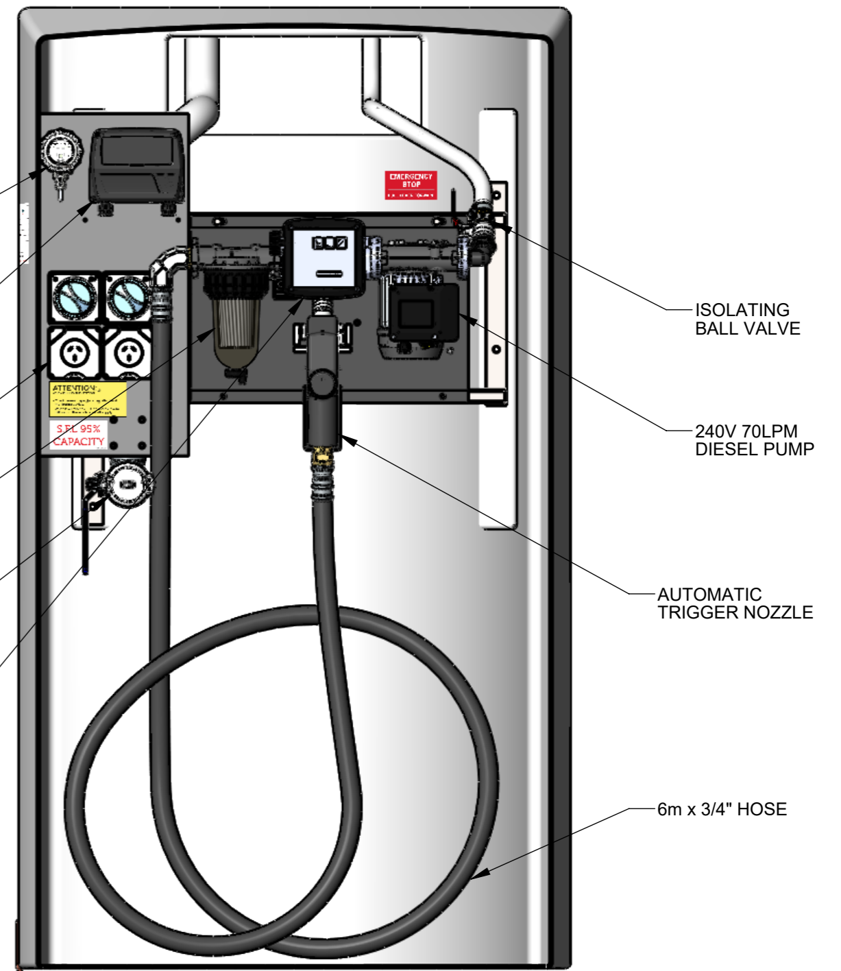
SECTION THRU CABINET FRONT SCALE 1 : 10
